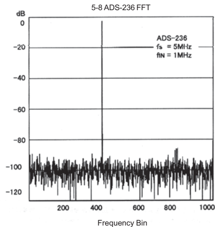
Figure 5. Typical Performance Curve
