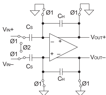
Figure 3.1 Analog Input Sample-and-Hold
