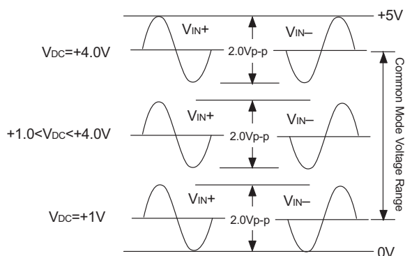
Figure 3.6 Differential Analog Input Common Mode Voltage Range
