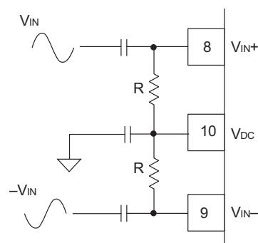
Figure 3.2 AC Coupled Differential Input
