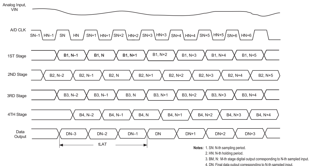
Figure 2A. Internal Timing Diagram
