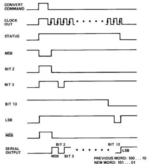
Figure 1. Timing Diagram
