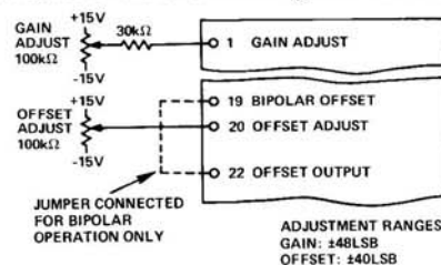
Figure 5. Adjustment Connections
