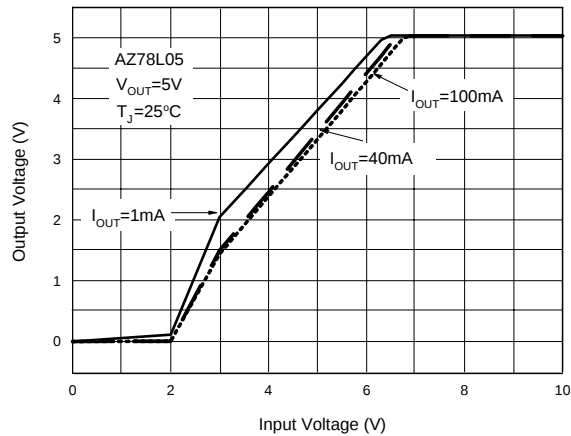
Figure 4. Dropout Characteristics
