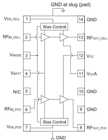
Figure 1: Block Diagram
